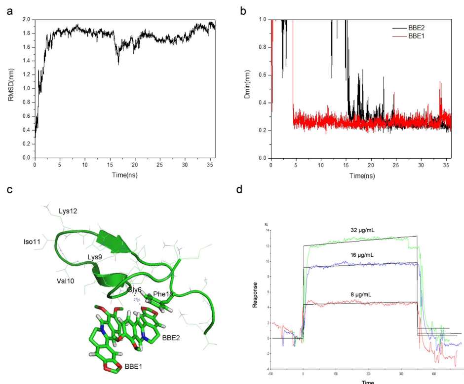
Figure 7. Interaction between berberine and PSMα2. (a) shows the backbone RMSD of PSMα2 during a 36 ns simulation. (b) The minimum distances between berberines (BBE1 and BBE2) and PSMα2 throughout the simulation. (c) The final structure of the simulation was visualized using the PyMOL Molecular Graphics System. (d) The association and dissociation of berberine with synthetic PSMα2 peptide was analyzed using SPR sensor chip.
